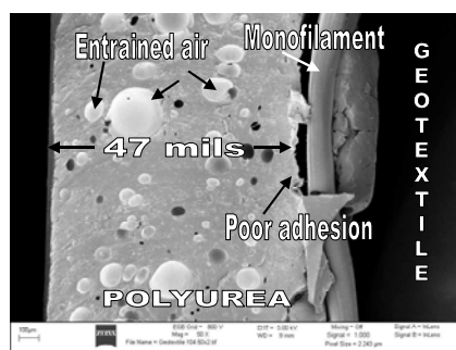
Figure 10: W-6 (woven, 50X).
